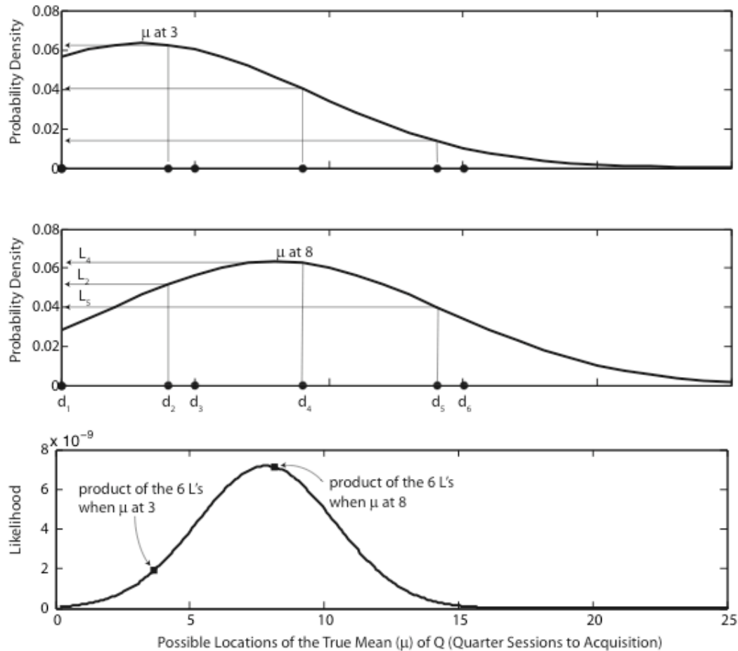
Figure 4. Computing a likelihood function. The assumed source distribution (the statistical model) is slid along the abscissa (here the \mu_Q axis), on which are plotted the known data (solid dots, labeled d_1 - d_6 in middle panel, which are the data from the Many&Dense group). The top two panels show it at two locations. At each location, the likelihoods are read off (arrows projecting up from 3 of the 6 data points and over to the corresponding probability densities). The product of the densities is the likelihood of that location (that value of \mu ), given the data. The likelihood function (bottom panel) is the plot of the likelihood as a function of the possible locations of the source distribution (possible values of \mu_Q ). Note that the area under the likelihood function is nowhere near one (numbers on ordinate of bottom panel are \times 10^9 ).
