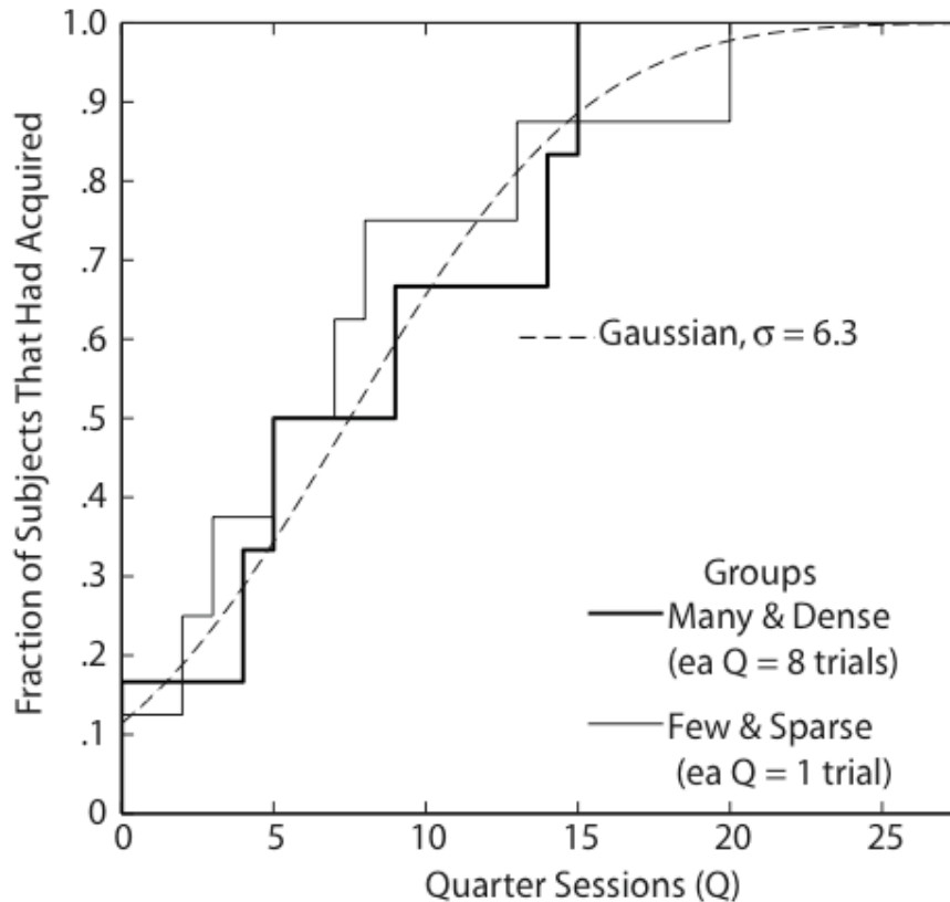
Figure 3. Cumulative distributions of quarter sessions to acquisition for two groups in Gottlieb's Experiment 4. These empirical cumulative distributions step up at the locus of each datum. Thus, the number of steps indicates the N ( N_{M\&D} = 6 ; N_{F\&S} = 8 ), and the location along the Q axis of any one step is the Q for one subject. The dashed curve is a cumulative Gaussian with a standard deviation of 6.3, which is the pooled maximum unbiased estimate of the standard deviation of the distribution from which the data are drawn (assuming that the source distributions have a common variance, but not necessarily a common mean).
