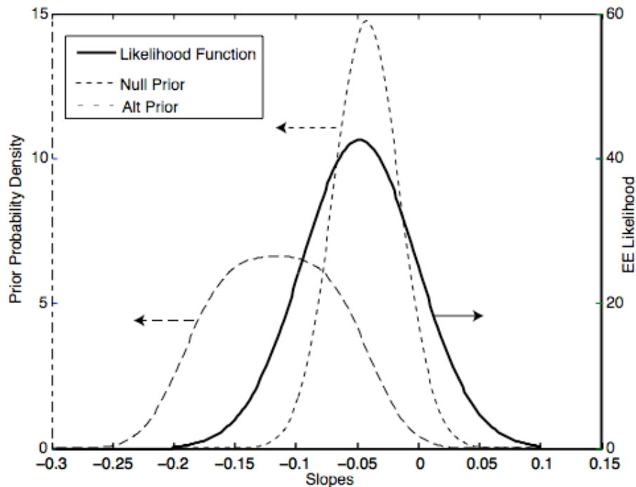
Figure 10. The null prior and convergence prior for the slope of the regression line through Subject 7's EE data (plotted against left axis), together with the likelihood function for the slope of those data (plotted against right axis).
