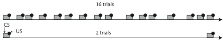
Figure 1. Schematic representation of (a portion of) two different classical conditioning protocols of equal duration but with an 8-fold difference in the number of trials (CS-US pairings) in a given amount of time ( t ). Gottlieb tested the hypothesis that these two protocols have equivalent effects on the progress of learning.
