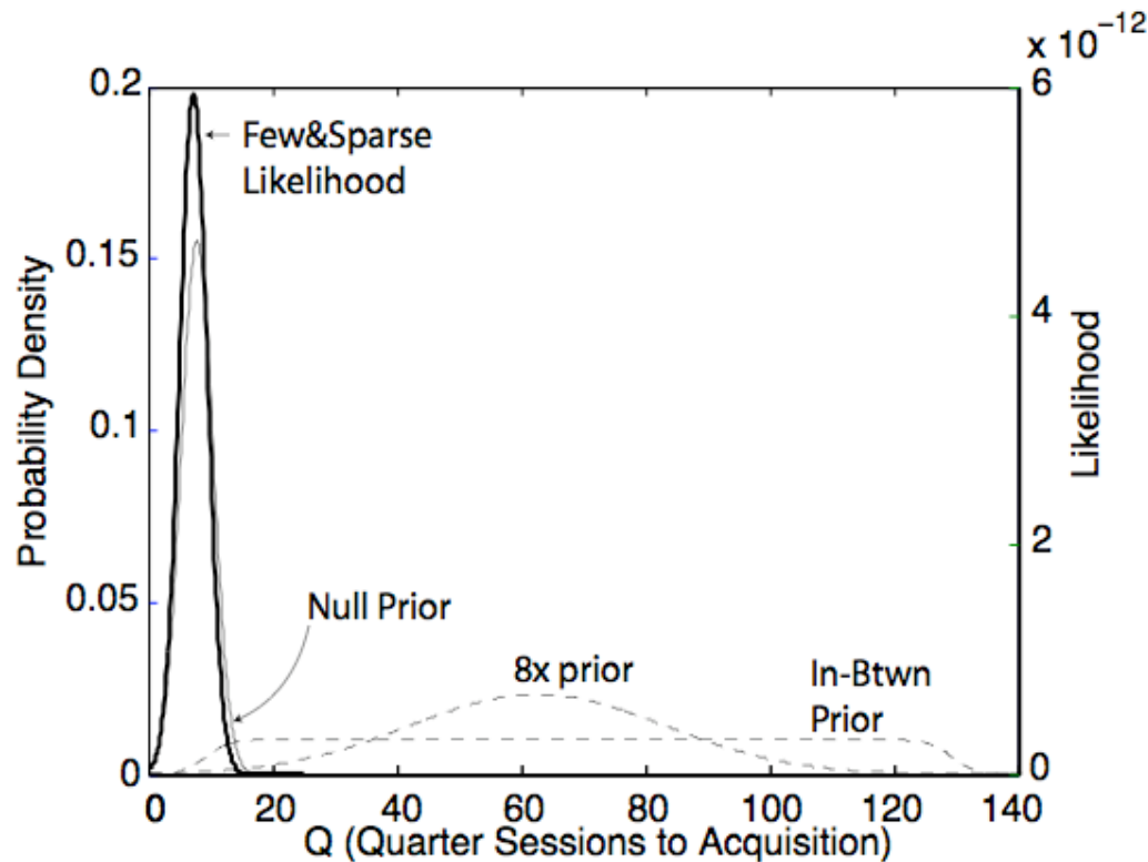
Figure 5. The likelihood function for the mean of the 1-trial-per-quarter-session group (heavy curve) and the three prior probability functions corresponding to three different hypotheses: 1) the null hypothesis, which is that the quarter-sessions-to-acquisition data from this group were drawn from the same distribution as the data from the 8-trials/quarter session group; 2) the 8x hypothesis which is that only trials matter, in which case the data from the 1-trial group were drawn from a distribution 8 times wider; 3) the vague hypothesis that the effect of reducing the number of trials per quarter session from 8 to 1 will have an effect somewhere within the range delimited by the null and the 8x hypotheses. The prior probability distributions are plotted against the left axis. They all, of course, integrate to 1. The likelihood function is plotted against the right axis; it does not integrate to 1.
